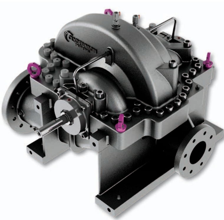
Pictured main: Duoglide-e horizontal arrangement
